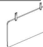
SEFJ08 600 * 350 * 8 800 * 350 * 8 1000 * 350 * 8 1400 * 350 * 8 1600 * 350 * 8 1800 * 350 * 8
